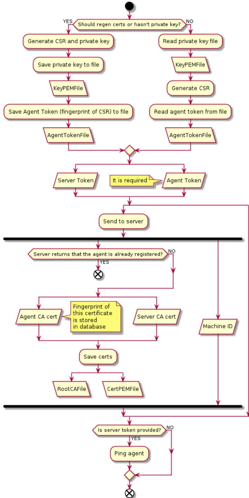
Fig. 1: Agent registration
